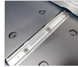
HELICAL-STYLE CUTTER HEAD W/ 16 TWO-SIDED CARBIDE INSERTS
