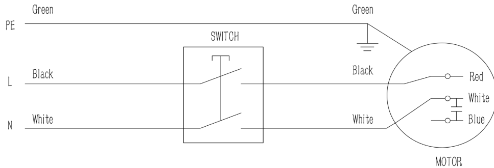
10-3062 Bandsaw - 1/2HP, 115V, 5.5A, 60Hz, 1Ph Motor
